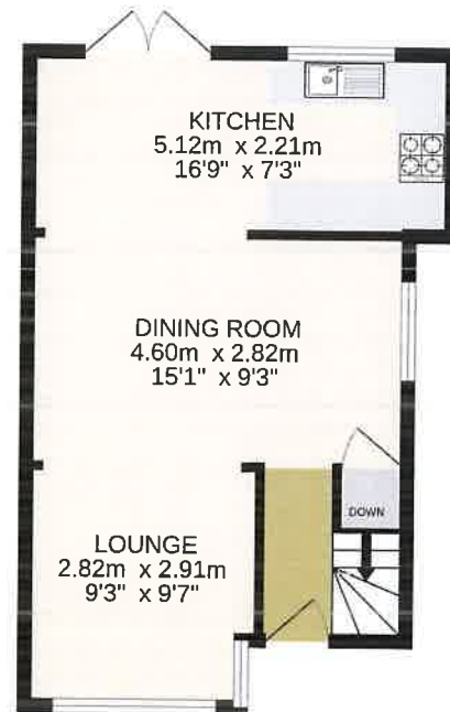
Ground floor 50.2 sq.m. (540 sq.ft.) approx.
